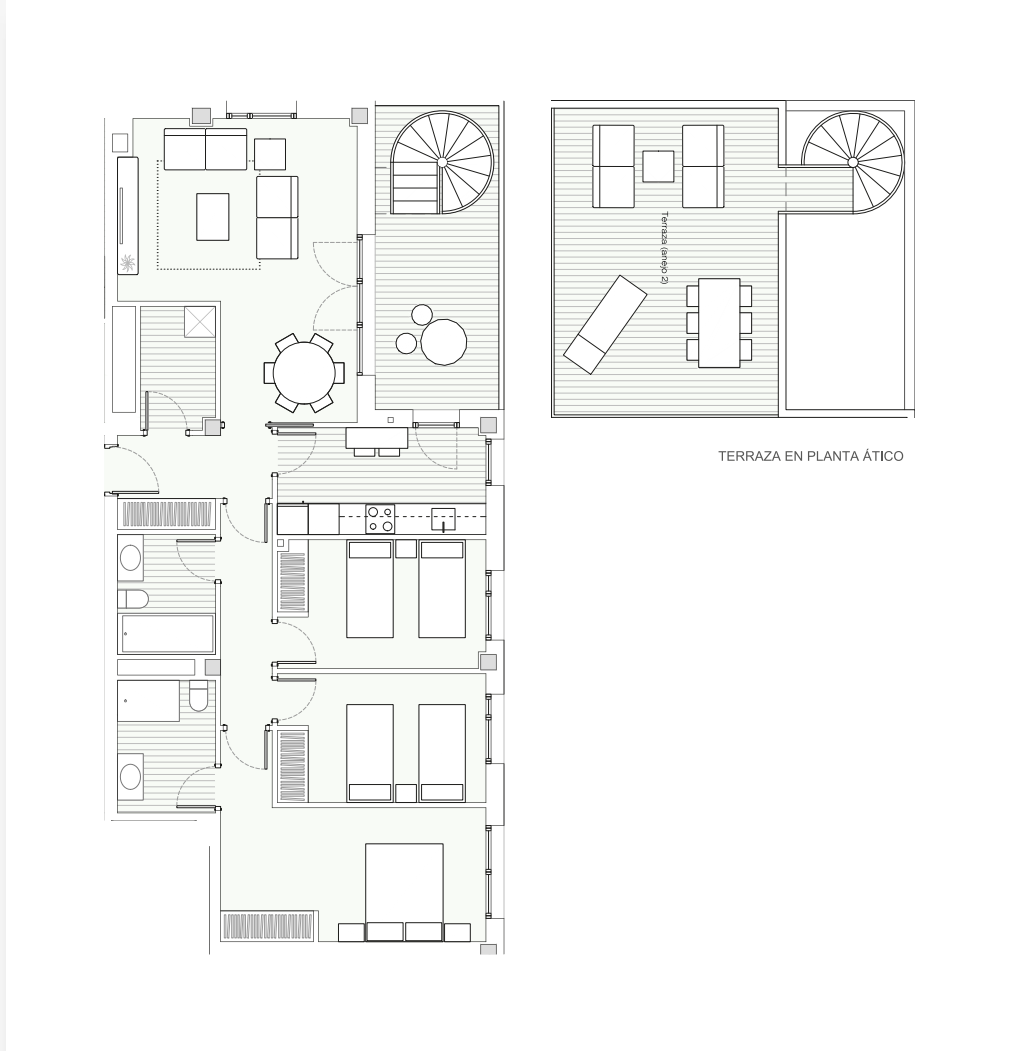
3-BEDROOM PENTHOUSE
